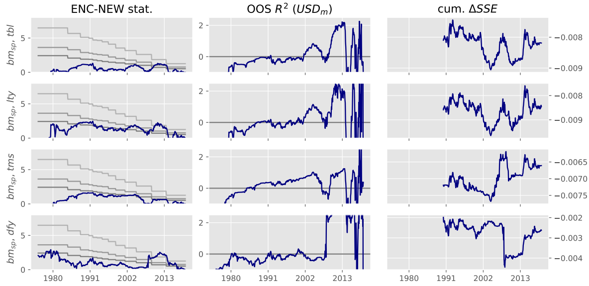
Figure 32: Recursive bivariate regressions of the equal-weighted dynamic dollar neutral carry trade strategy on selected regressors.
